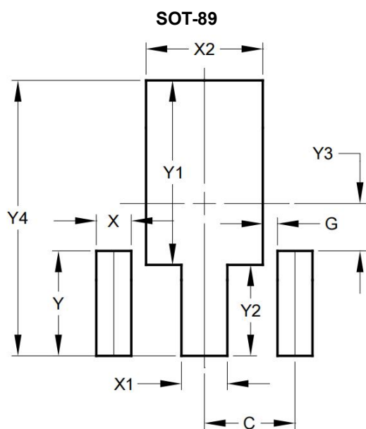
Fig. Soldering footprint for SOT-89
